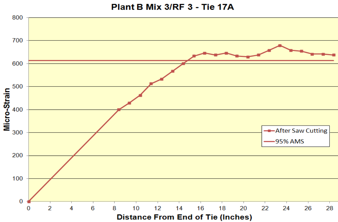
Figure B.19: Transfer length of Plant B Mix 3/RF 3 Tie 17A
