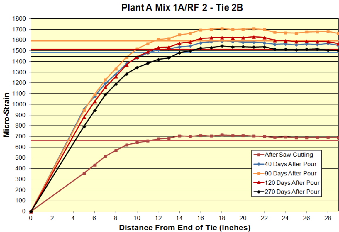
Figure A.46: Transfer length of Plant A Mix 1A/RF 2 Tie 2B
