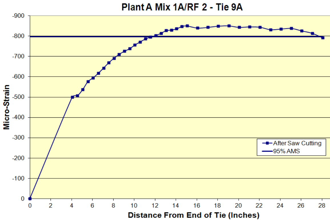
Figure A.39: Transfer length of Plant A Mix 1A/RF 2 Tie 9A
