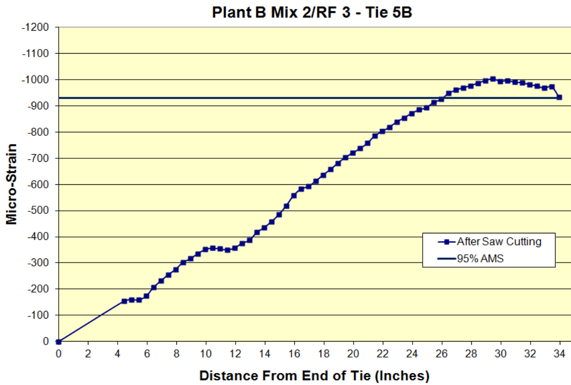
Figure B.6: Transfer length of Plant B Mix 2/RF 3 Tie 5B
