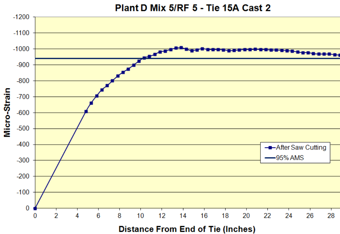
Figure D.14: Transfer length of Plant D Mix 5/RF 5 Tie 15A Cast 2
