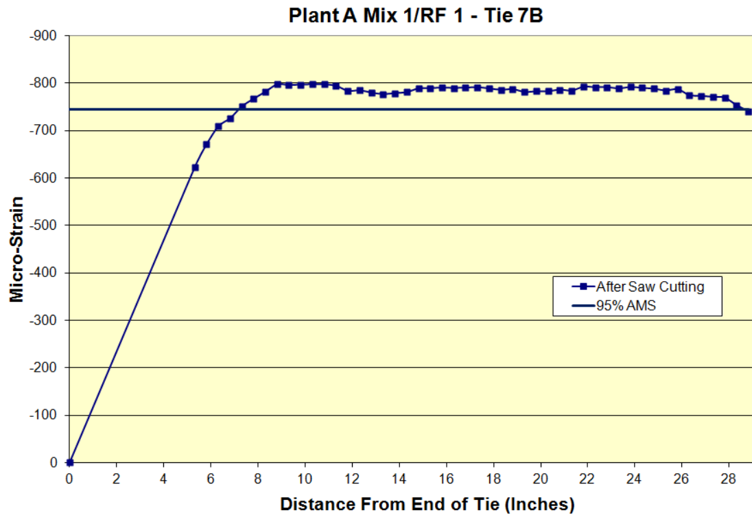
Figure A.7: Transfer length of Plant A Mix 1/RF 1 Tie 7B
