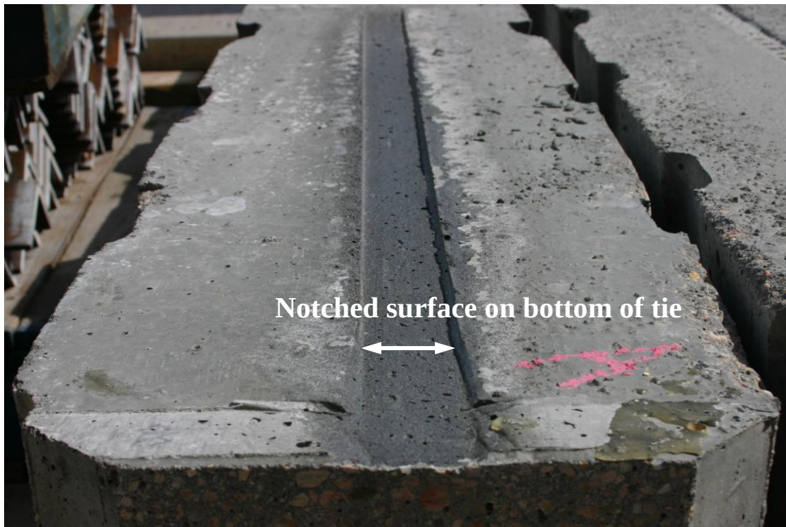
Figure 3.15: Notch created by steel bar inserts
