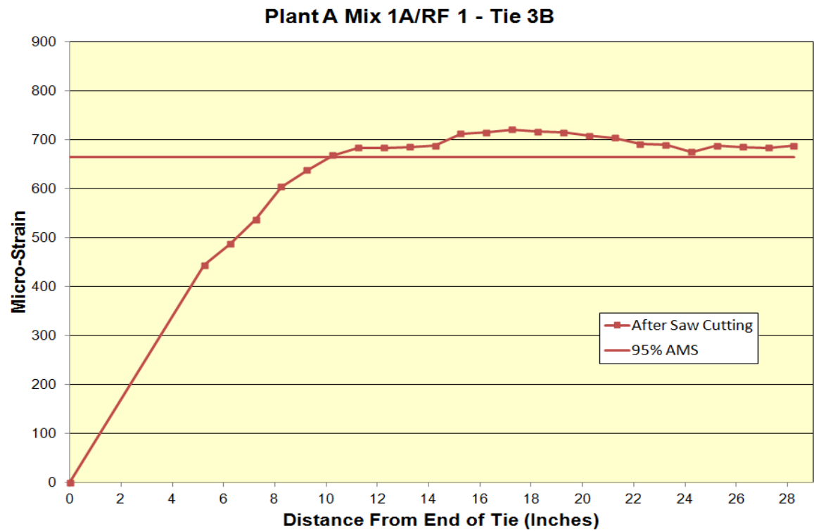
Figure A.22: Transfer length of Plant A Mix 1A/RF 1 Tie 3B
