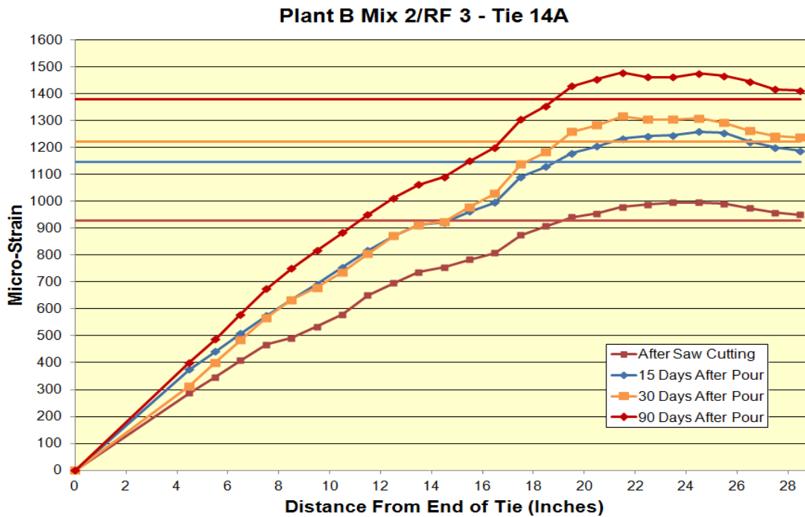
Figure B.43: Long-term transfer length of Plant B Mix 2/RF 3 Tie 14A
