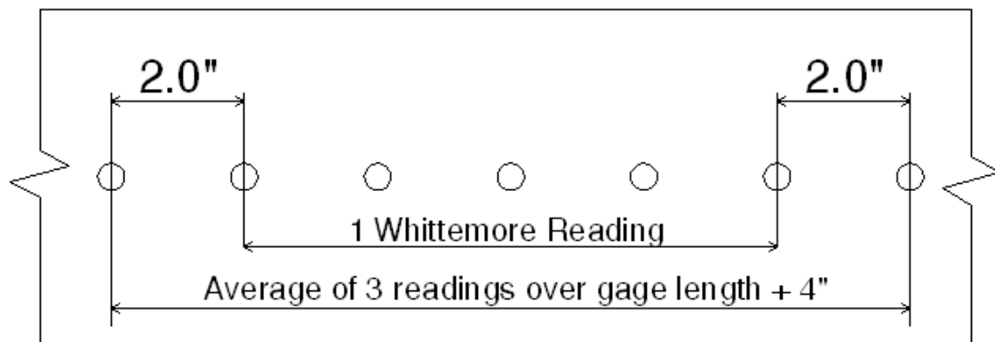
Figure 4.4: 12-inch length created using the 3-point average method
