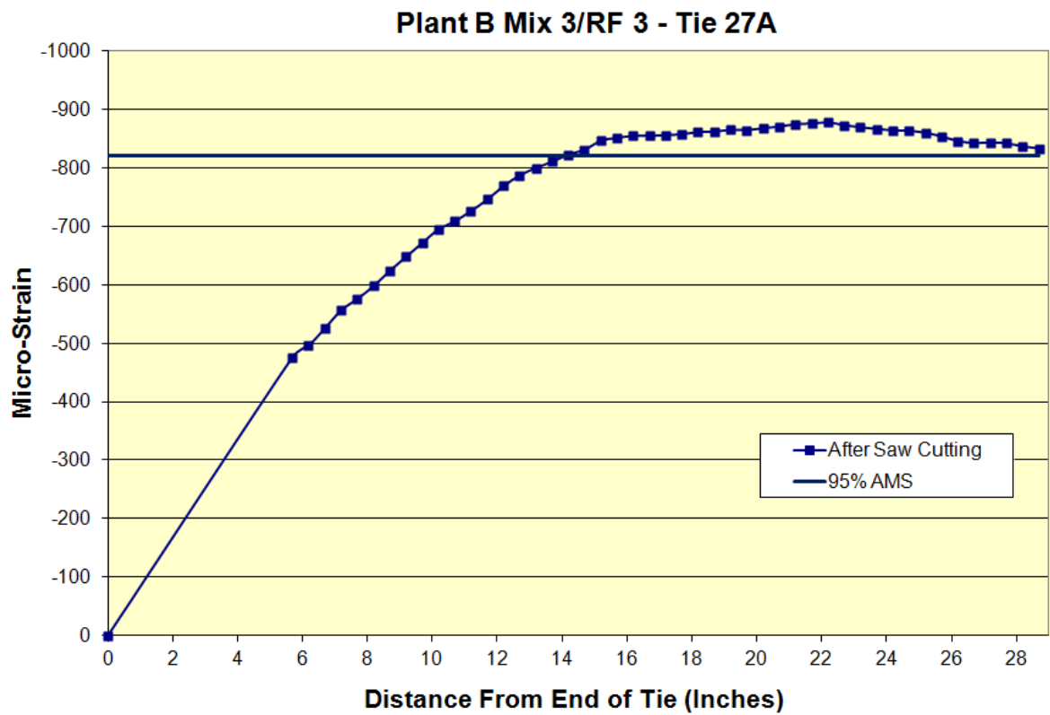
Figure B.36: Transfer length of Plant B Mix 3/RF 3 Tie 27A
