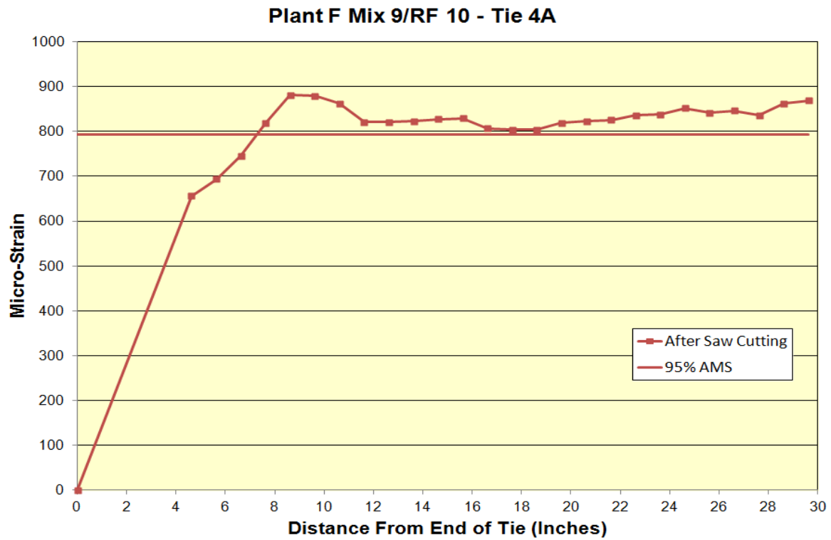
Figure F.33: Transfer length of Plant F Mix 9/RF 10 Tie 4A
