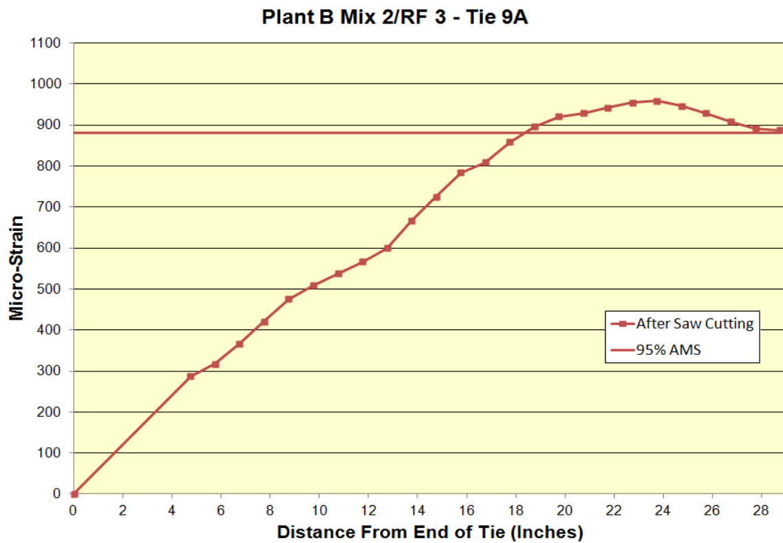
Figure B.11: Transfer length of Plant B Mix 2/RF 3 Tie 9A
