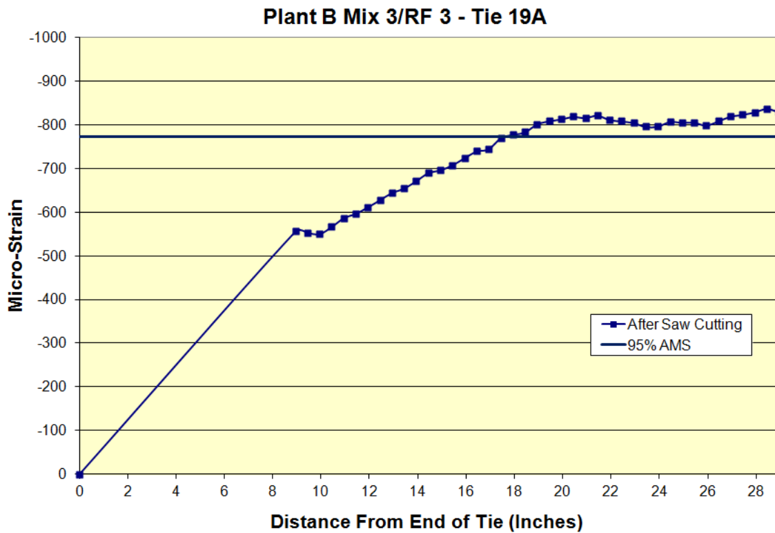
Figure B.23: Transfer length of Plant B Mix 3/RF 3 Tie 19A
