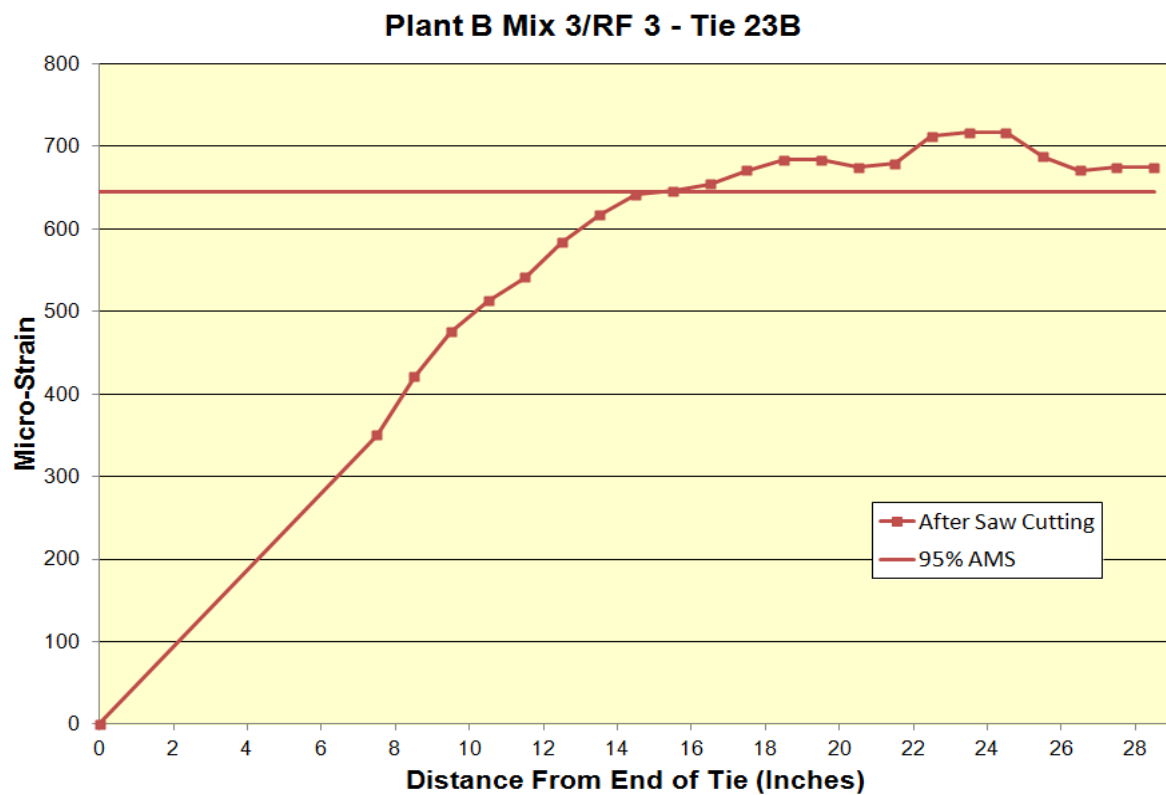
Figure B.30: Transfer length of Plant B Mix 3/RF 3 Tie 23B
