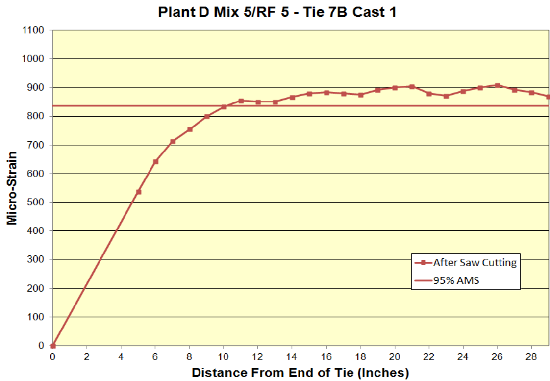
Figure D.5: Transfer length of Plant D Mix 5/RF 5 Tie 7B Cast 1
