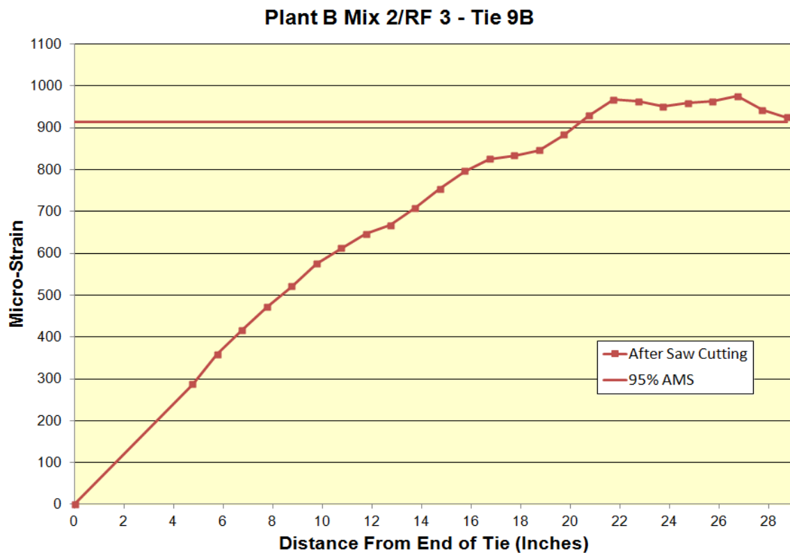
Figure B.12: Transfer length of Plant B Mix 2/RF 3 Tie 9B
