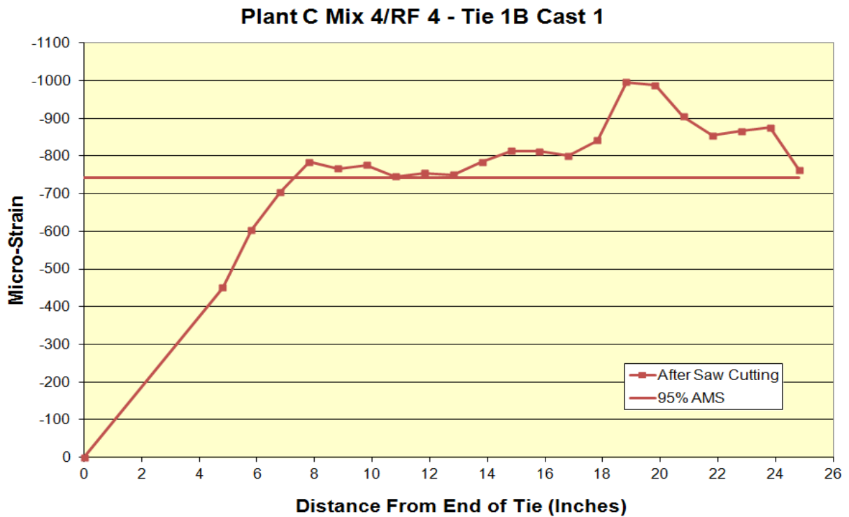
Figure C.2: Transfer length of Plant C Mix 4/RF 4 Tie 1B Cast 1
