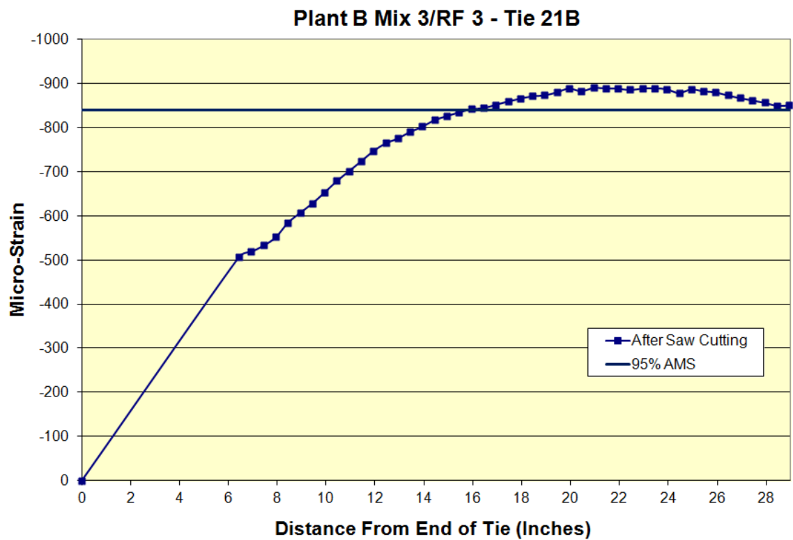
Figure B.28: Transfer length of Plant B Mix 3/RF 3 Tie 21B
