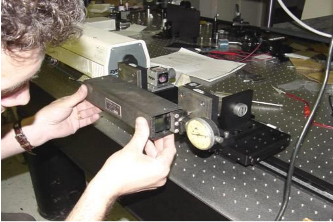
Figure 3.3: Determining accuracy of a standard mechanical gage (Zhao, 2011)
