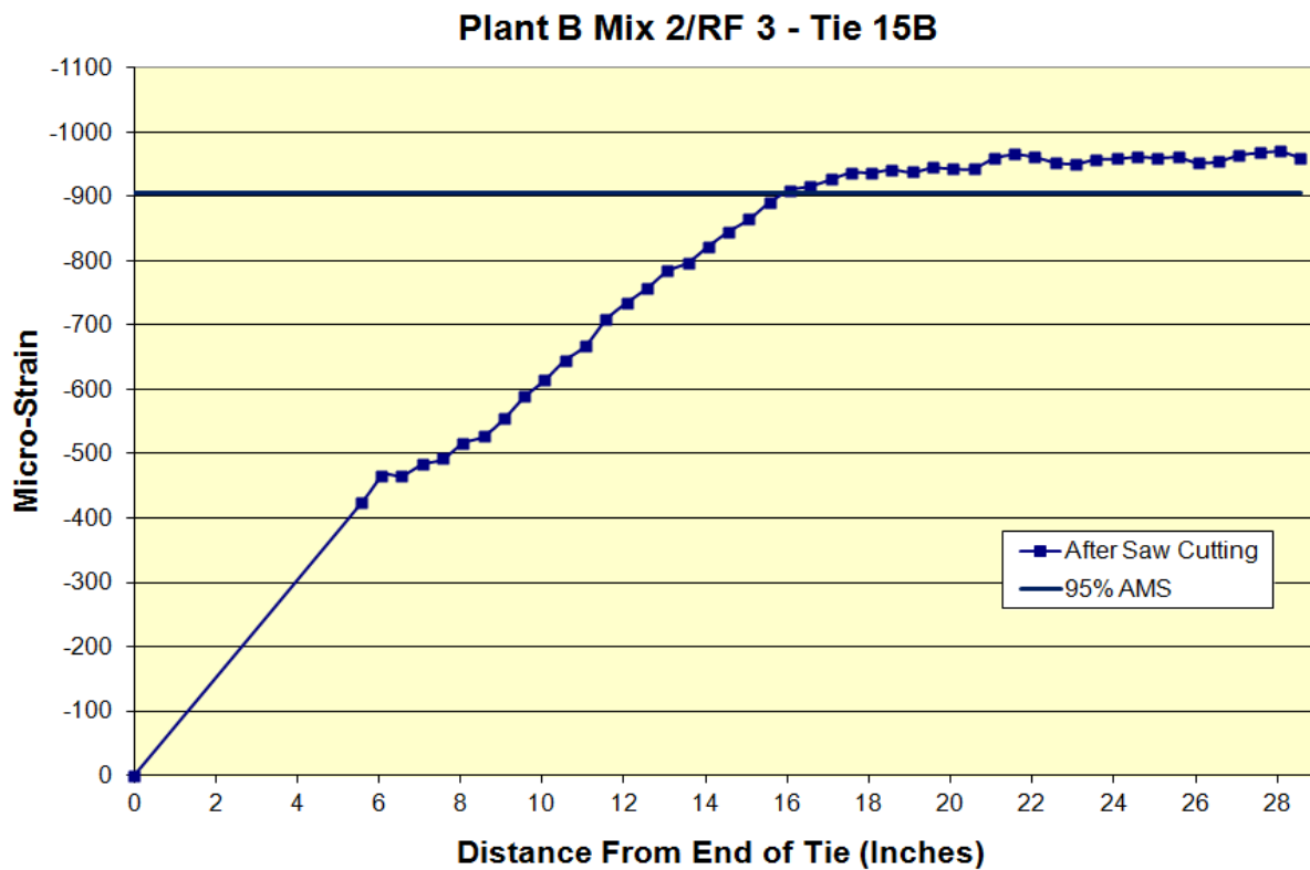
Figure B.18: Transfer length of Plant B Mix 2/RF 3 Tie 15B
