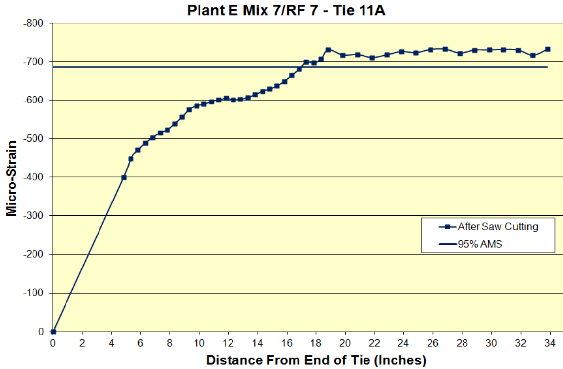
Figure E.19: Transfer length of Plant E Mix 7/RF 7 Tie 11A
