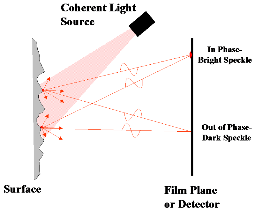
Figure 3.1: Illustration of the laser-speckle concept (Zhao, 2011)
