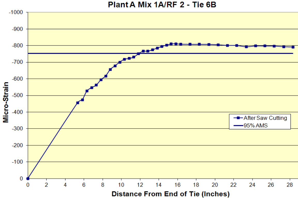
Figure A.38: Transfer length of Plant A Mix 1A/RF 2 Tie 6B
