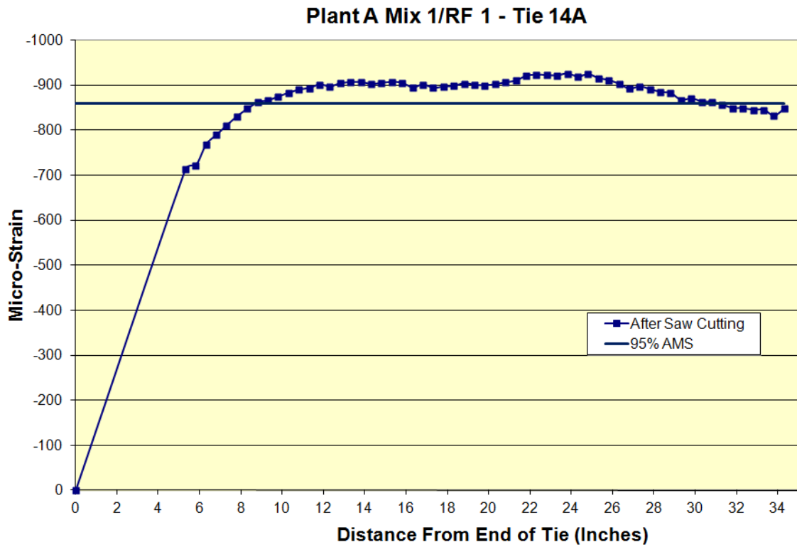
Figure A.15: Transfer length of Plant A Mix 1/RF 1 Tie 14A
