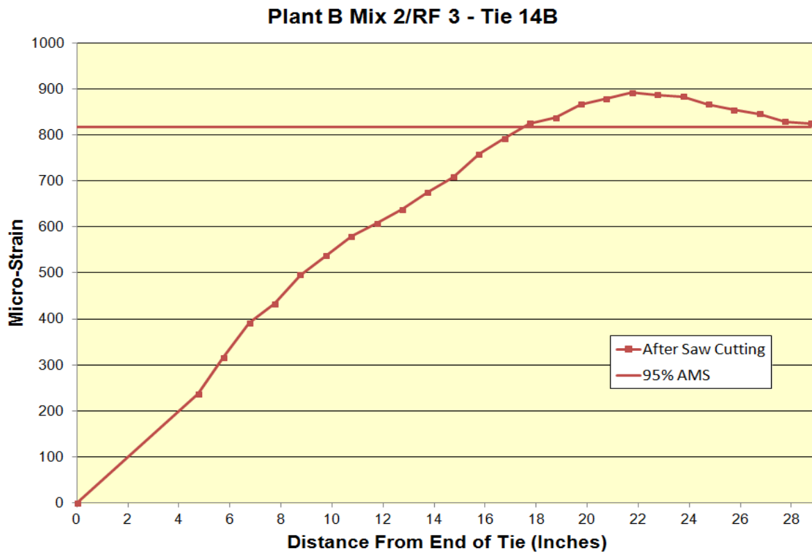
Figure B.17: Transfer length of Plant B Mix 2/RF 3 Tie 14B
