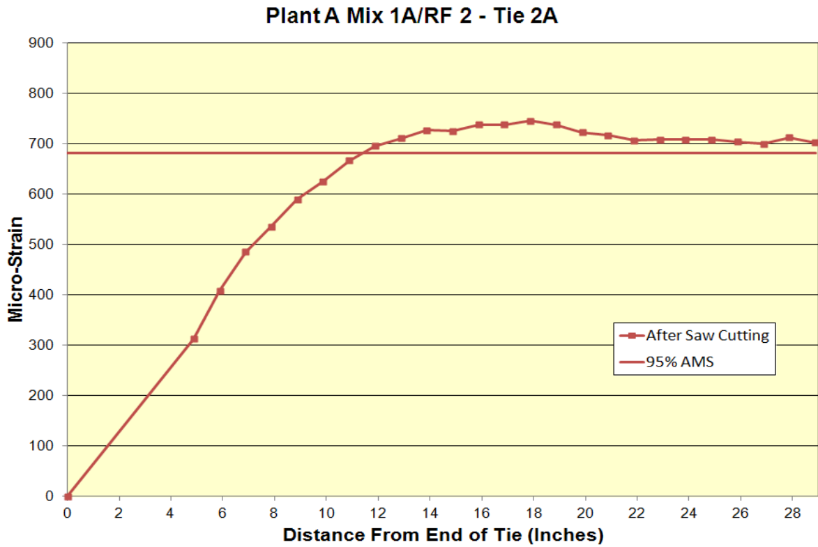
Figure A.33: Transfer length of Plant A Mix 1A/RF 2 Tie 2A
