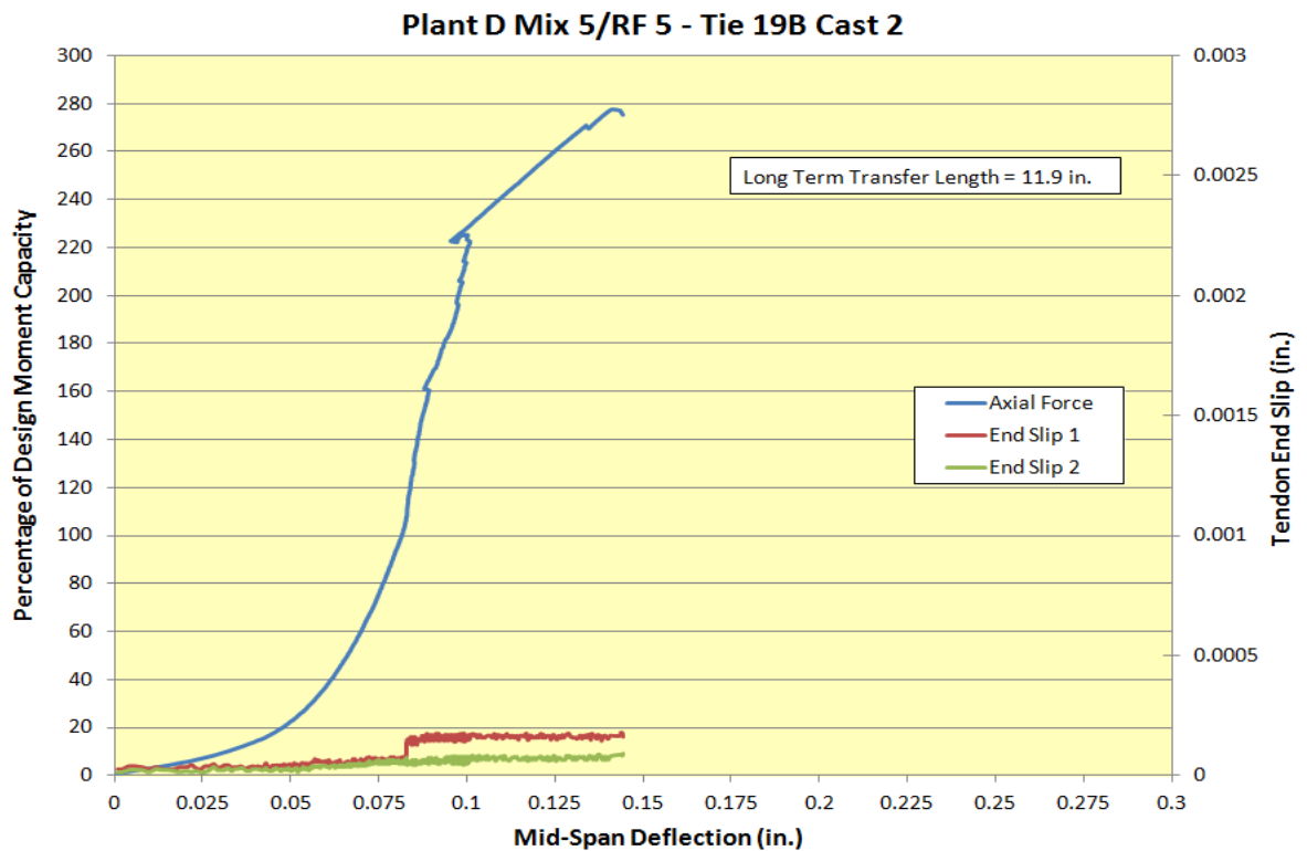
Figure 7.19: Load test results of Plant D Mix 5/RF 5 Tie 19B Cast 2
