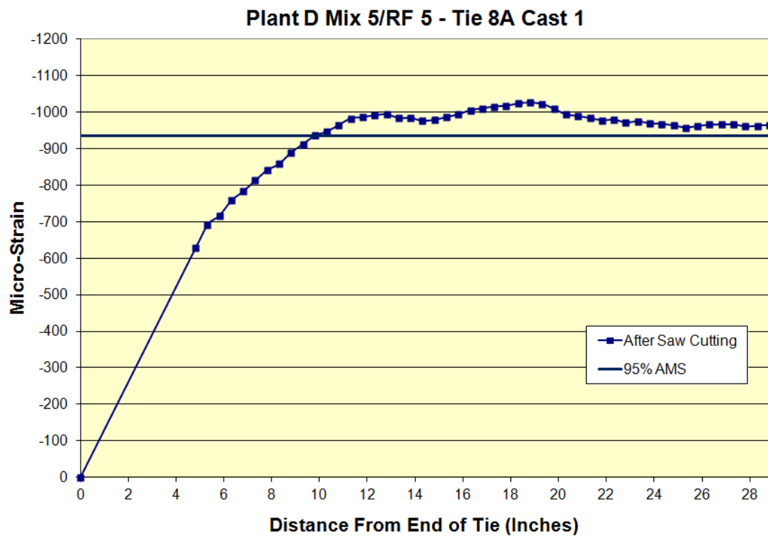
Figure D.6: Transfer length of Plant D Mix 5/RF 5 Tie 8A Cast 1
