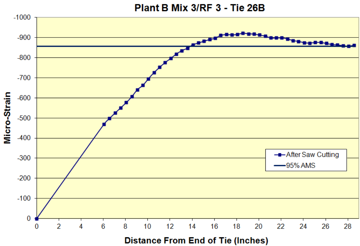
Figure B.35: Transfer length of Plant B Mix 3/RF 3 Tie 26B
