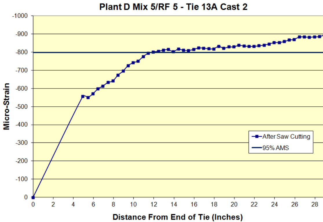
Figure D.11: Transfer length of Plant D Mix 5/RF 5 Tie 13A Cast 2
