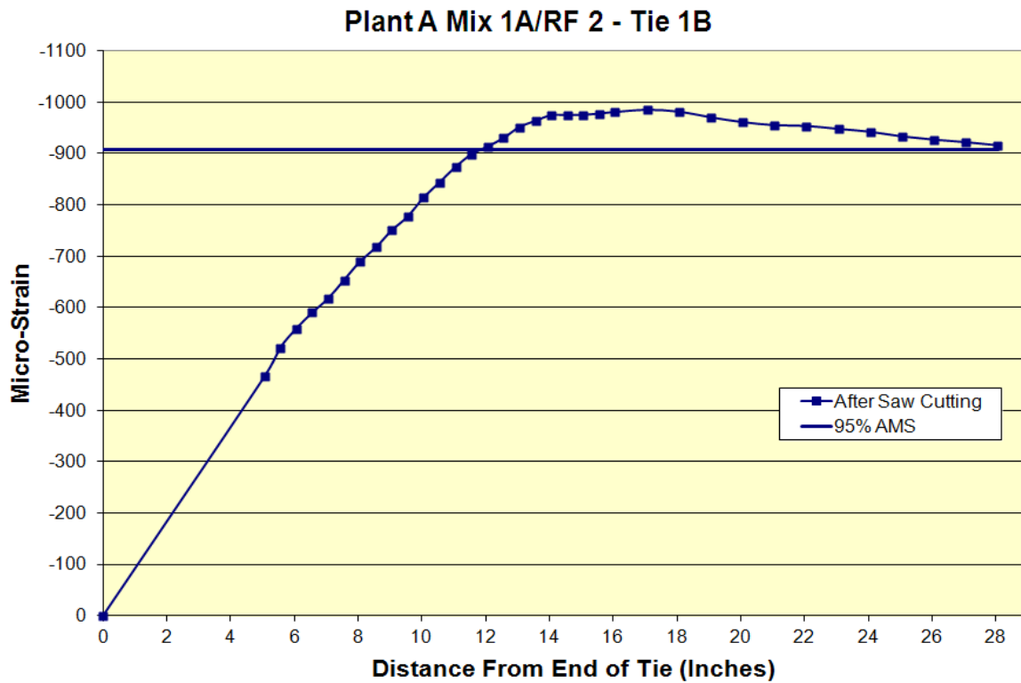
Figure A.32: Transfer length of Plant A Mix 1A/RF 2 Tie 1B
