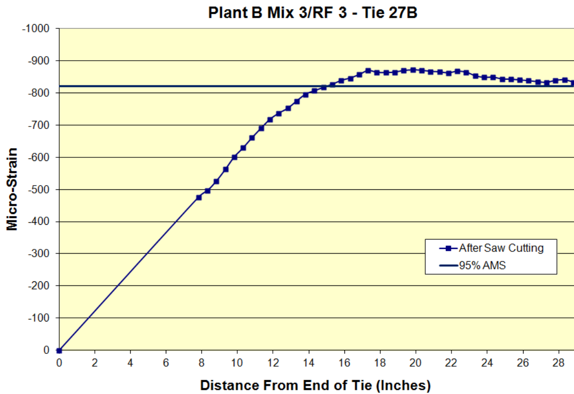
Figure B.37: Transfer length of Plant B Mix 3/RF 3 Tie 27B
