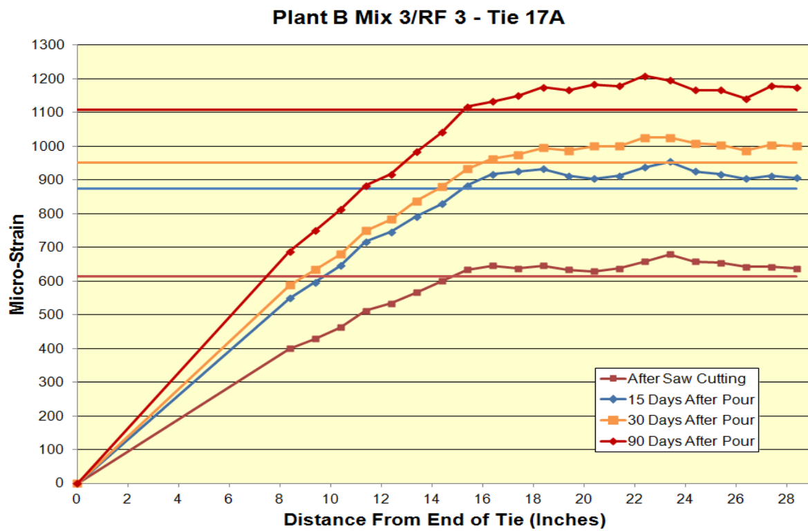
Figure B.45: Long-term transfer length of Plant B Mix 3/RF 3 Tie 17A
