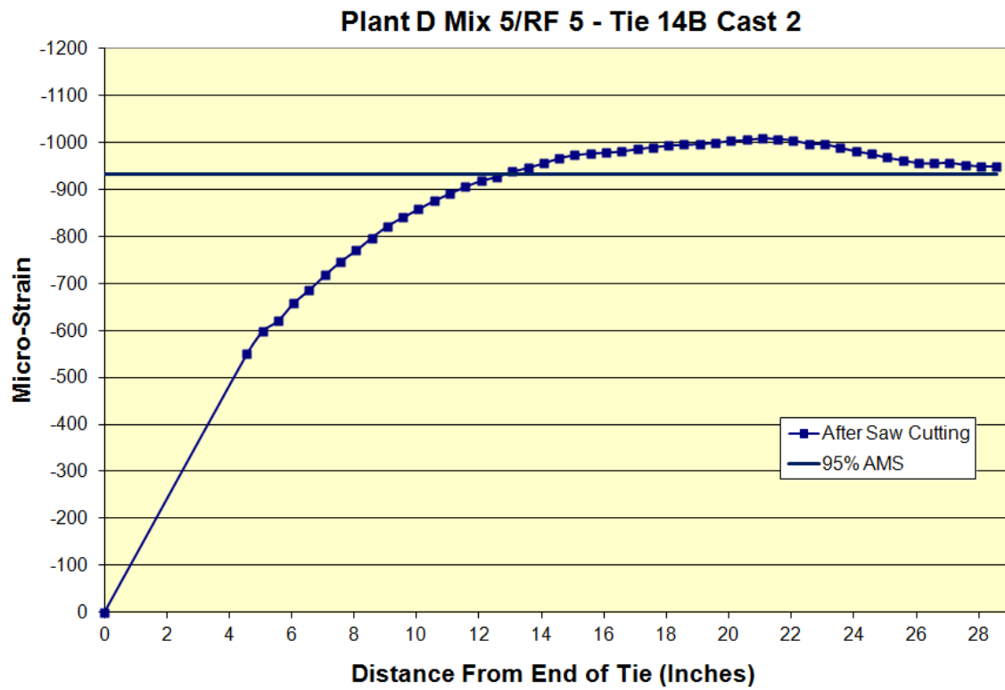
Figure D.13: Transfer length of Plant D Mix 5/RF 5 Tie 14B Cast 2
