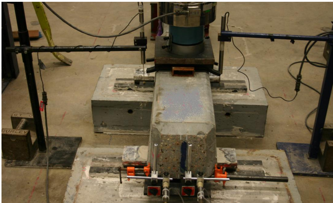
Figure 7.5: Setup of rail seat positive moment test
