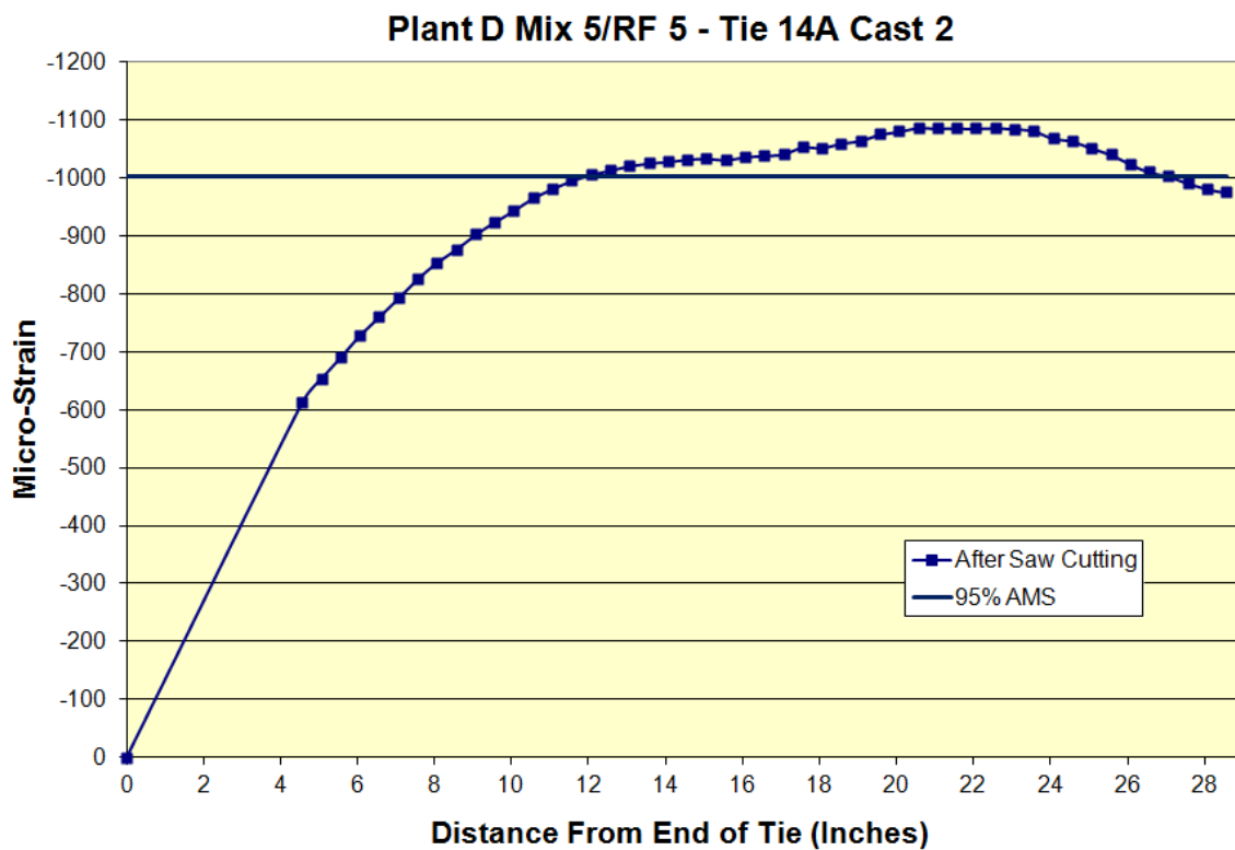
Figure D.12: Transfer length of Plant D Mix 5/RF 5 Tie 14A Cast 2
