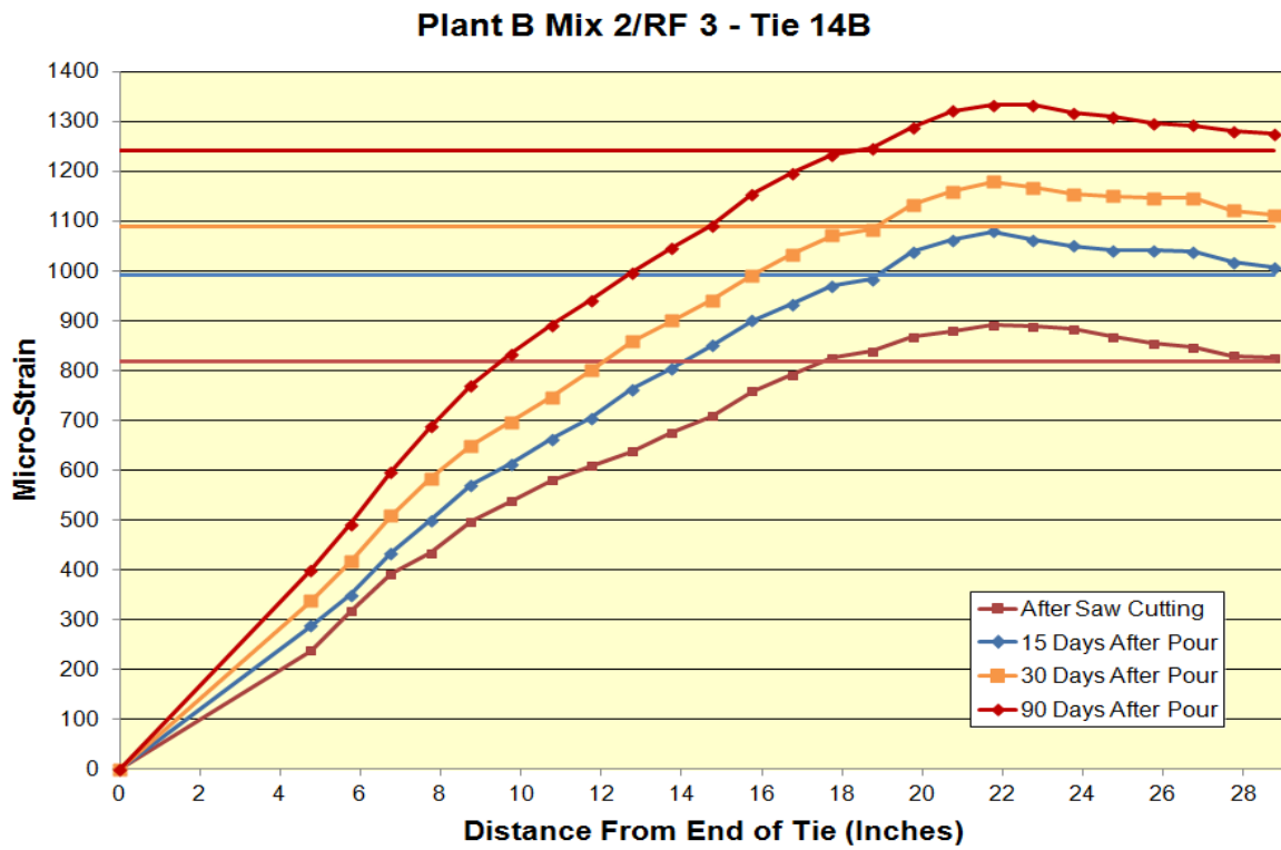
Figure B.44: Long-term transfer length of Plant B Mix 2/RF 3 Tie 14B
