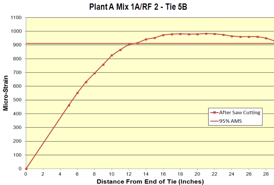
Figure A.36: Transfer length of Plant A Mix 1A/RF 2 Tie 5B
