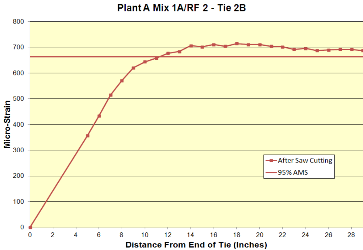
Figure A.34: Transfer length of Plant A Mix 1A/RF 2 Tie 2B
