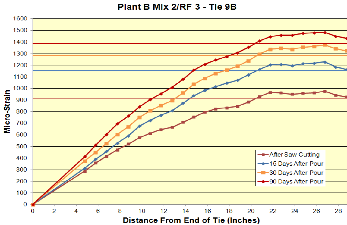
Figure B.42: Long-term transfer length of Plant B Mix 2/RF 3 Tie 9B
