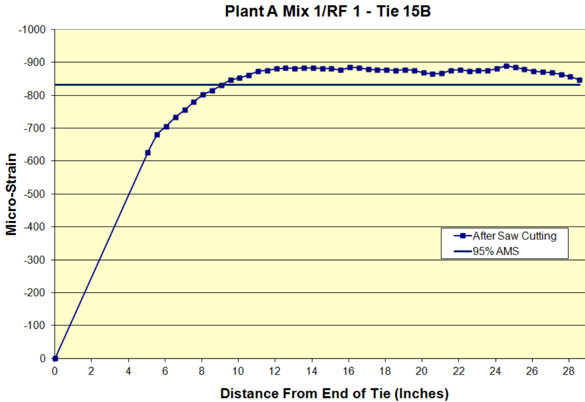
Figure A.16: Transfer length of Plant A Mix 1/RF 1 Tie 15B
