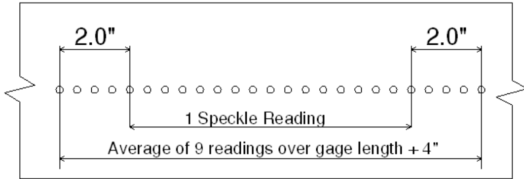
Figure 4.5: 12-inch length created using the 9-point average method
