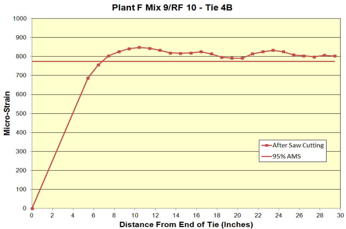
Figure F.34: Transfer length of Plant F Mix 9/RF 10 Tie 4B
