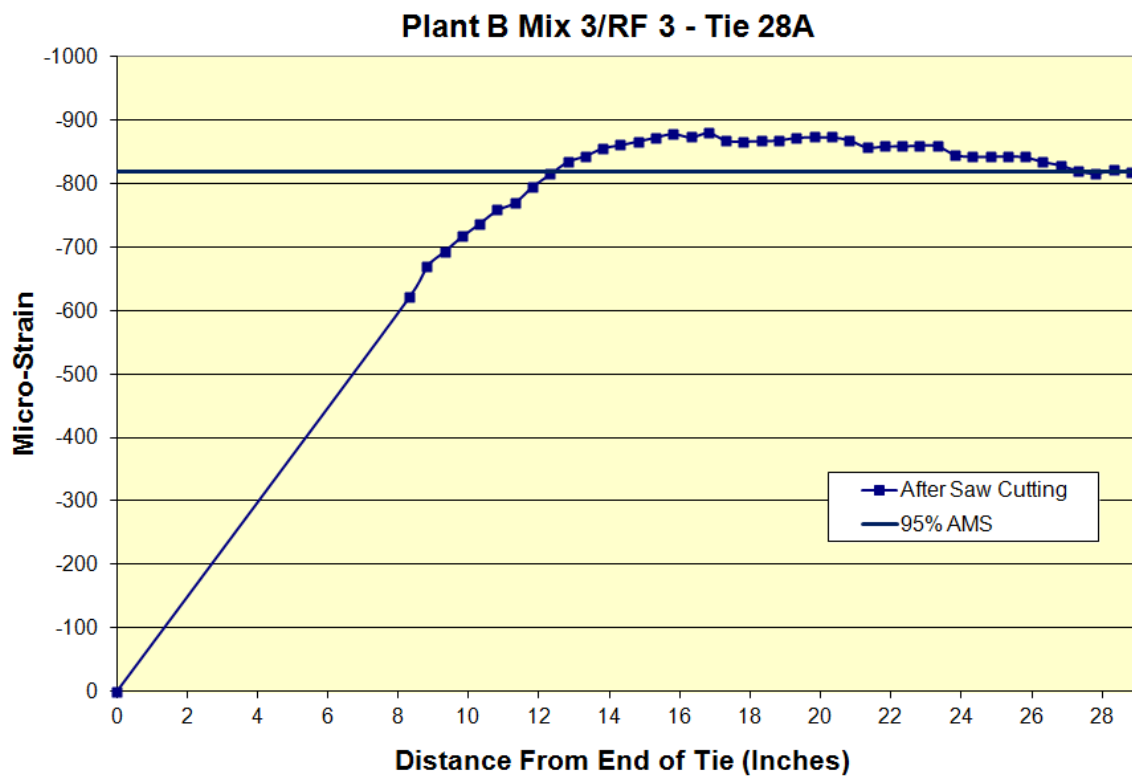
Figure B.38: Transfer length of Plant B Mix 3/RF 3 Tie 28A
