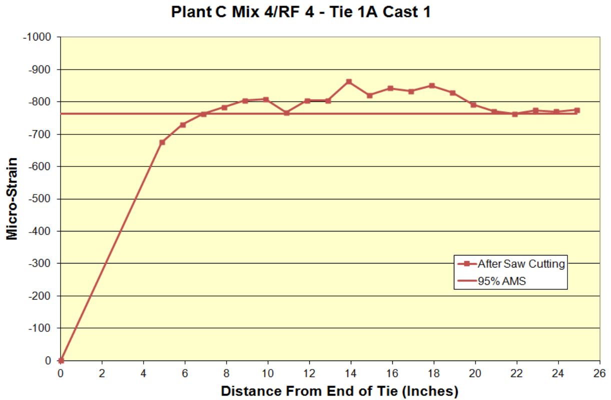
Figure C.1: Transfer length of Plant C Mix 4/RF 4 Tie 1A Cast 1
