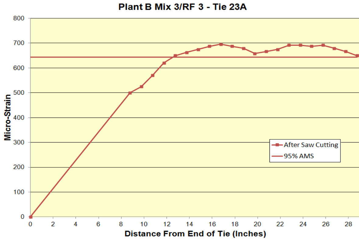
Figure B.29: Transfer length of Plant B Mix 3/RF 3 Tie 23A
