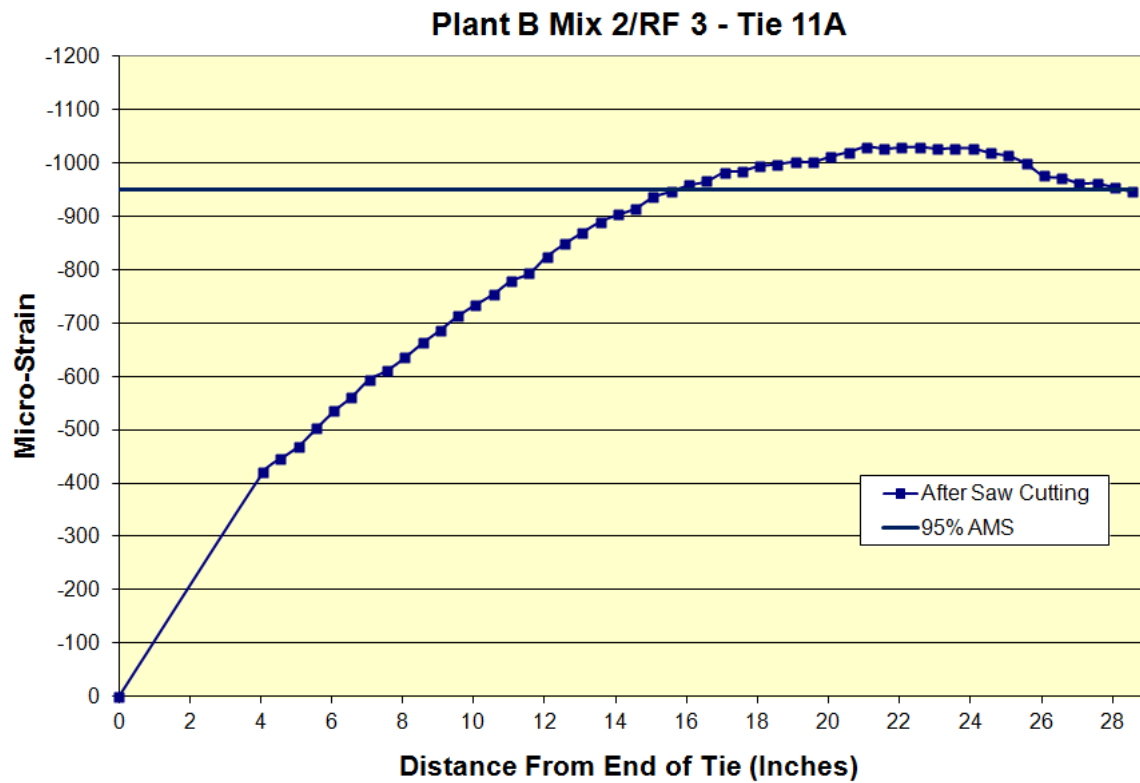
Figure B.13: Transfer length of Plant B Mix 2/RF 3 Tie 11A
