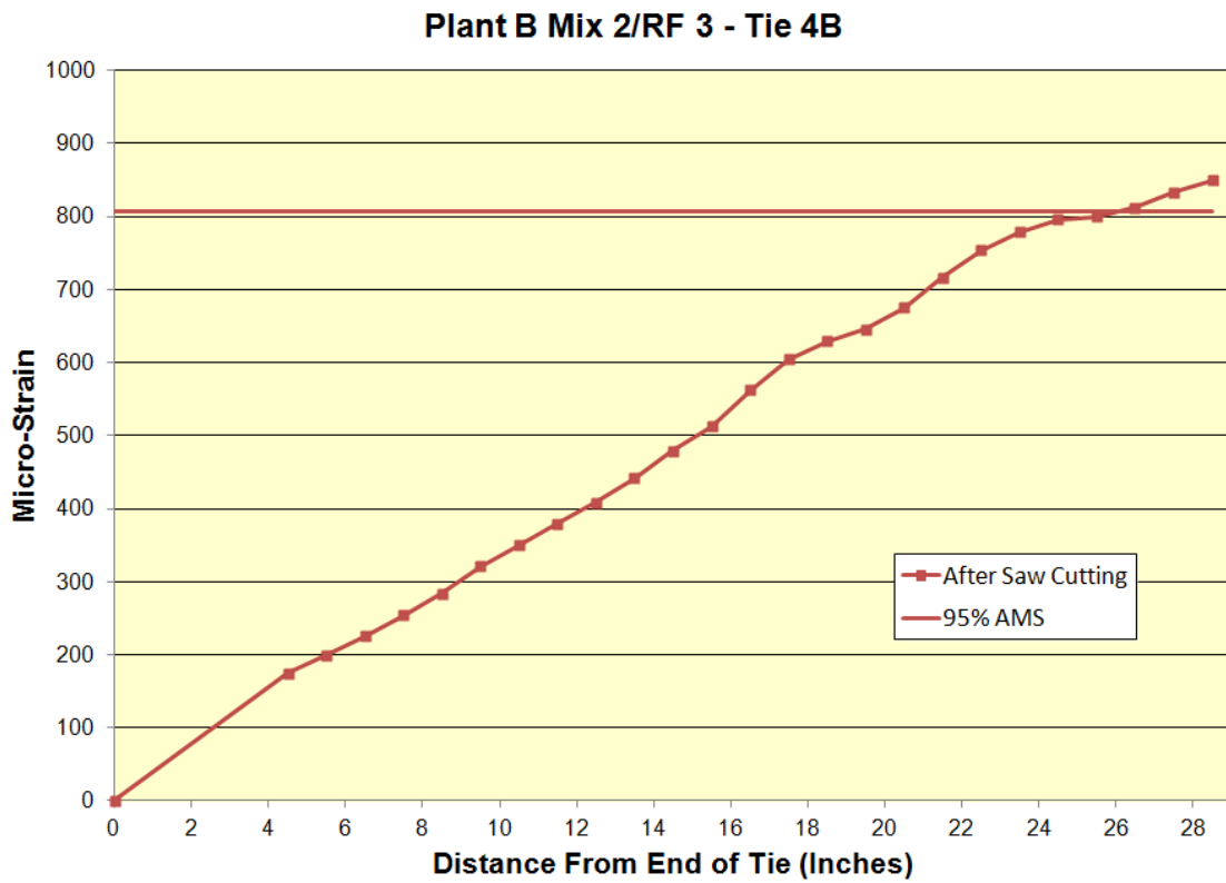
Figure B.5: Transfer length of Plant B Mix 2/RF 3 Tie 4B
