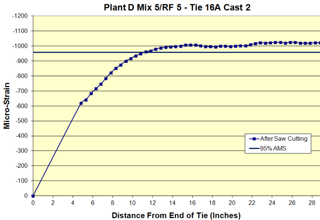
Figure D.16: Transfer length of Plant D Mix 5/RF 5 Tie 16A Cast 2
