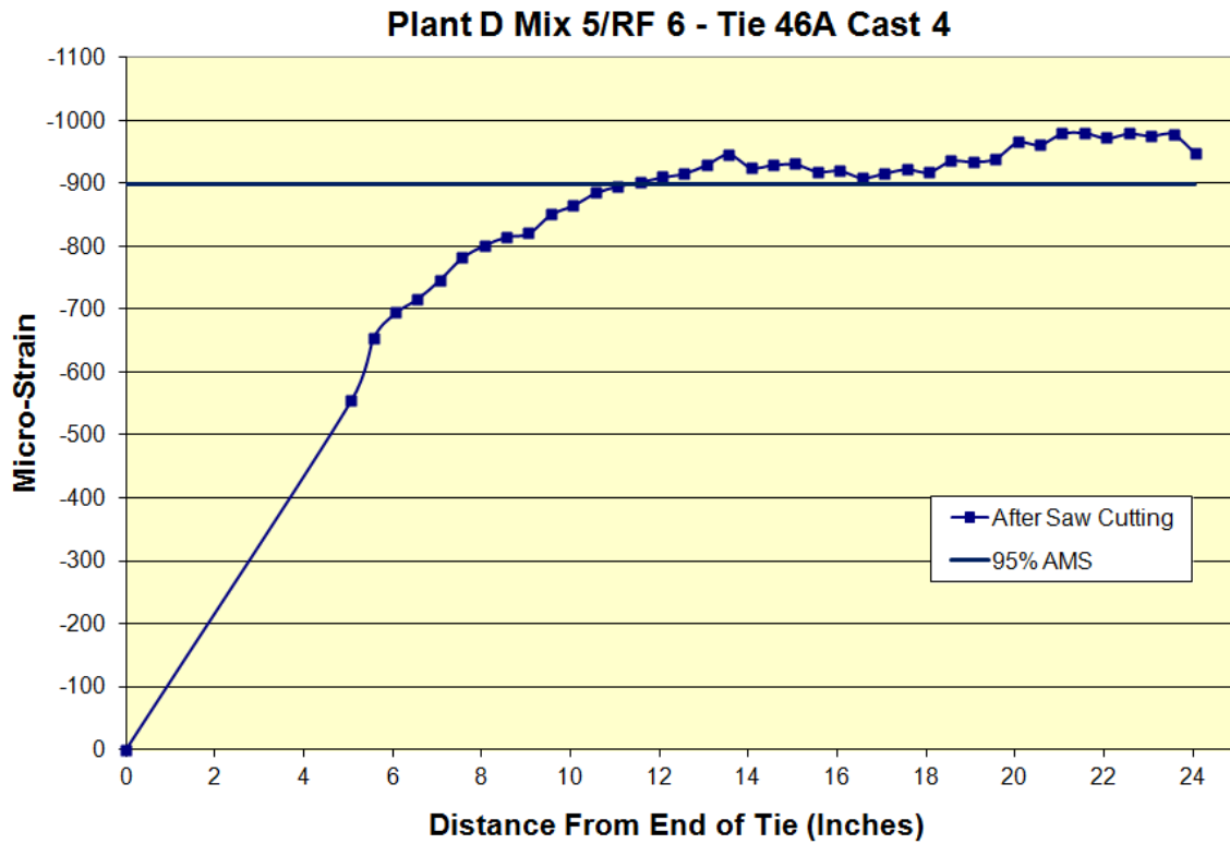
Figure D.61: Transfer length of Plant D Mix 5/RF 6 Tie 46A Cast 4
