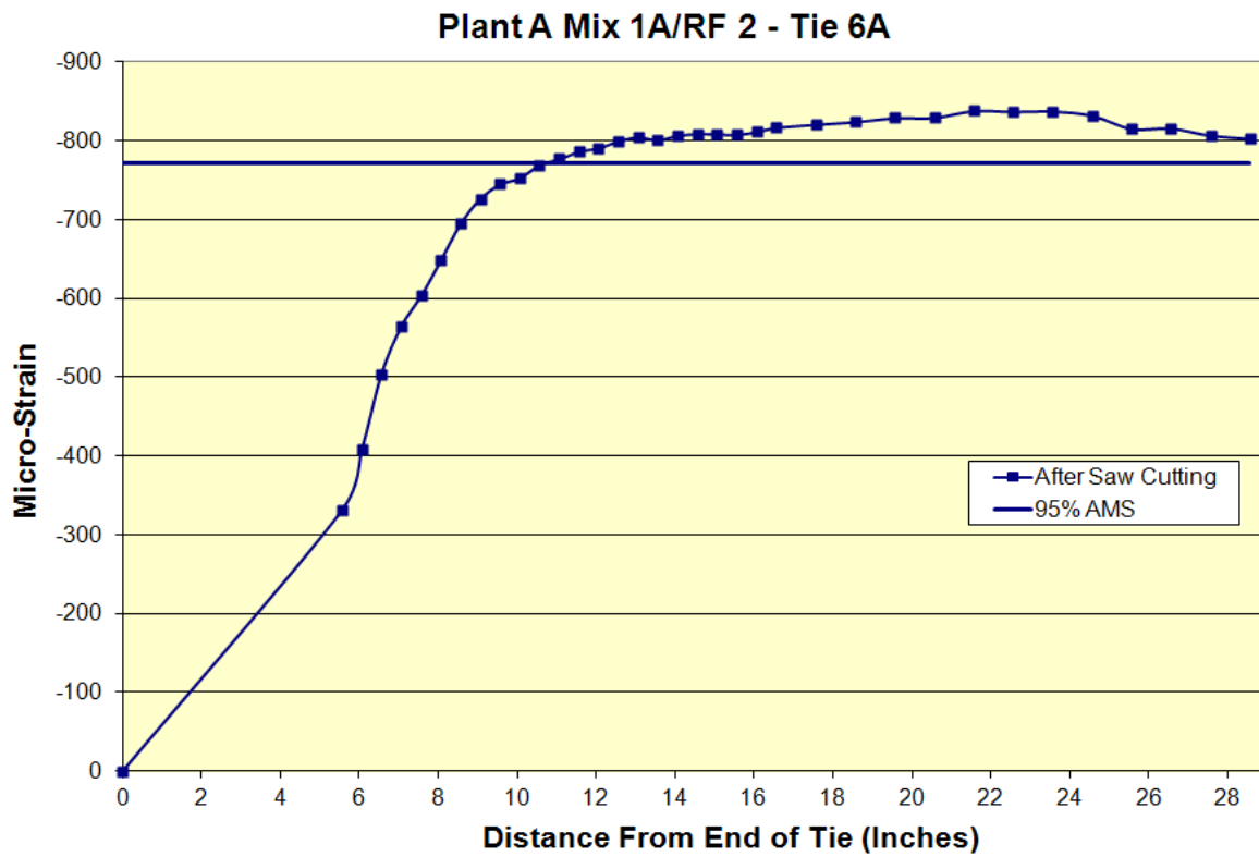
Figure A.37: Transfer length of Plant A Mix 1A/RF 2 Tie 6A
