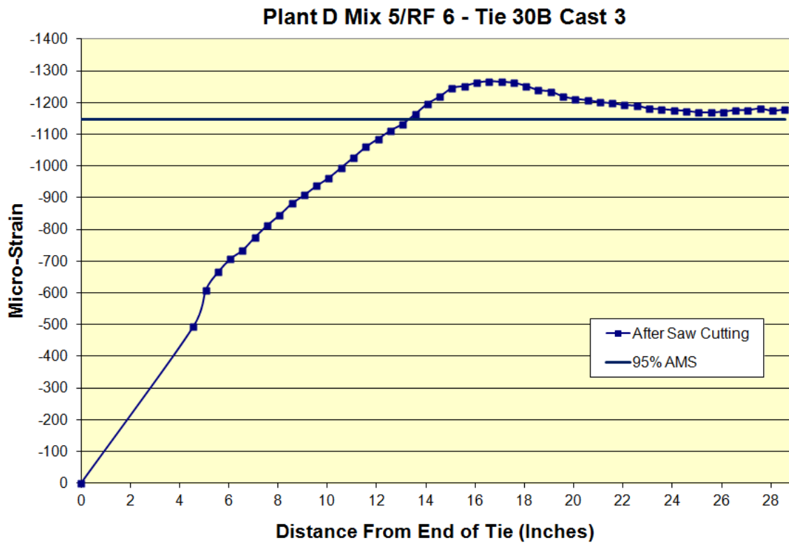
Figure D.33: Transfer length of Plant D Mix 5/RF 6 Tie 30B Cast 3
