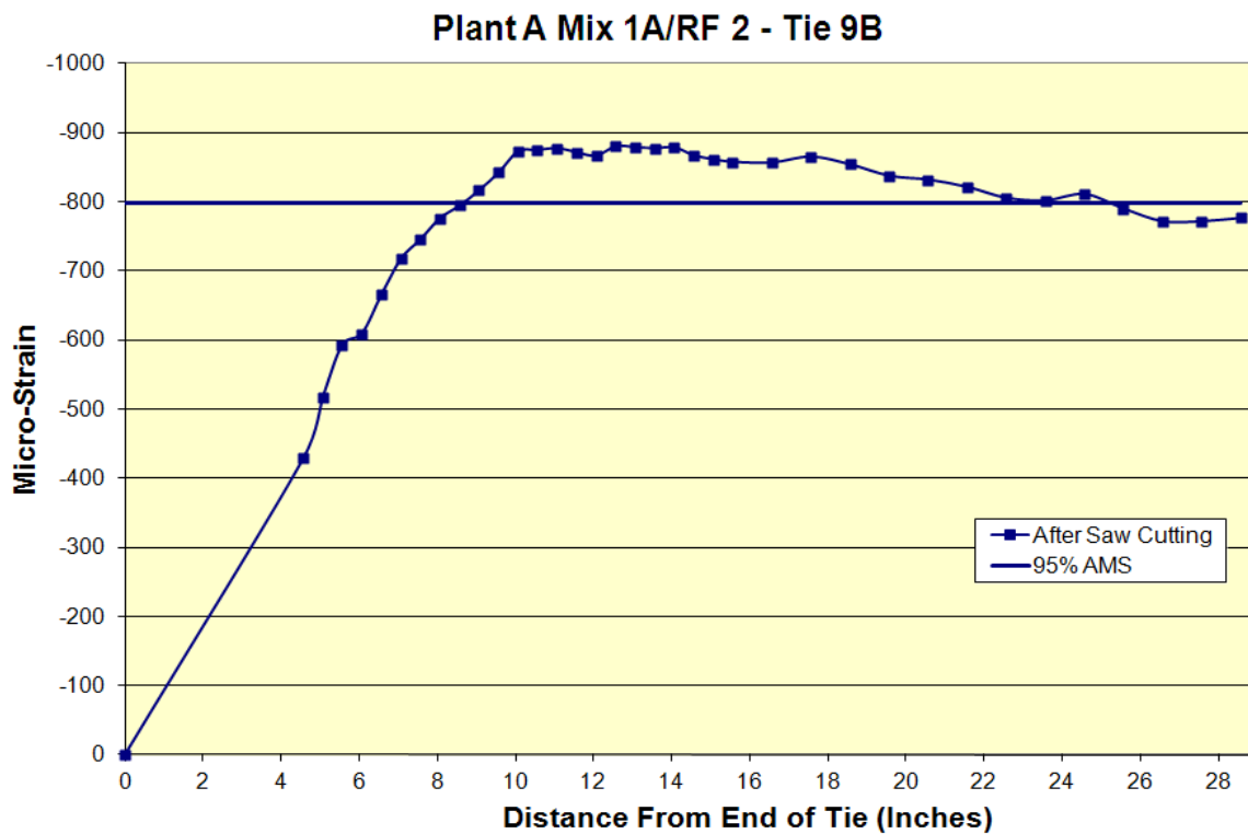
Figure A.40: Transfer length of Plant A Mix 1A/RF 2 Tie 9B
