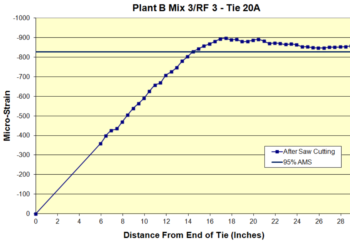
Figure B.25: Transfer length of Plant B Mix 3/RF 3 Tie 20A
