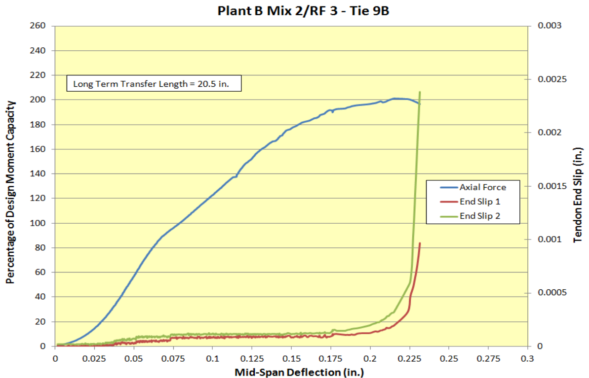
Figure 7.11: Load test results of Plant B Mix 2/RF 3 Tie 9B
