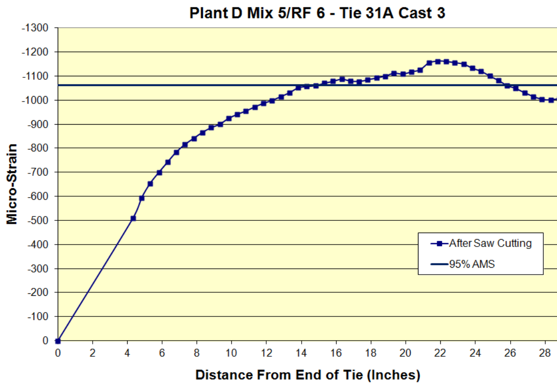
Figure D.34: Transfer length of Plant D Mix 5/RF 6 Tie 31A Cast 3
