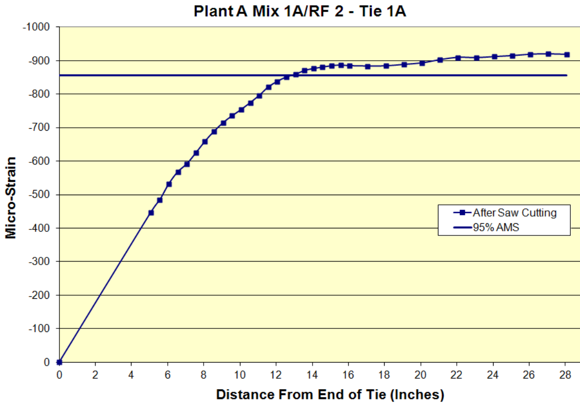
Figure A.31: Transfer length of Plant A Mix 1A/RF 2 Tie 1A
