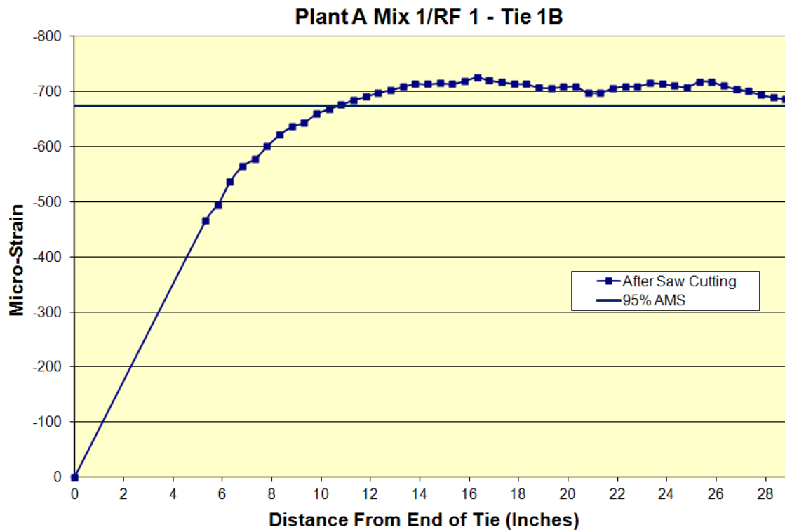
Figure A.1: Transfer length of Plant A Mix 1/RF 1 Tie 1B
